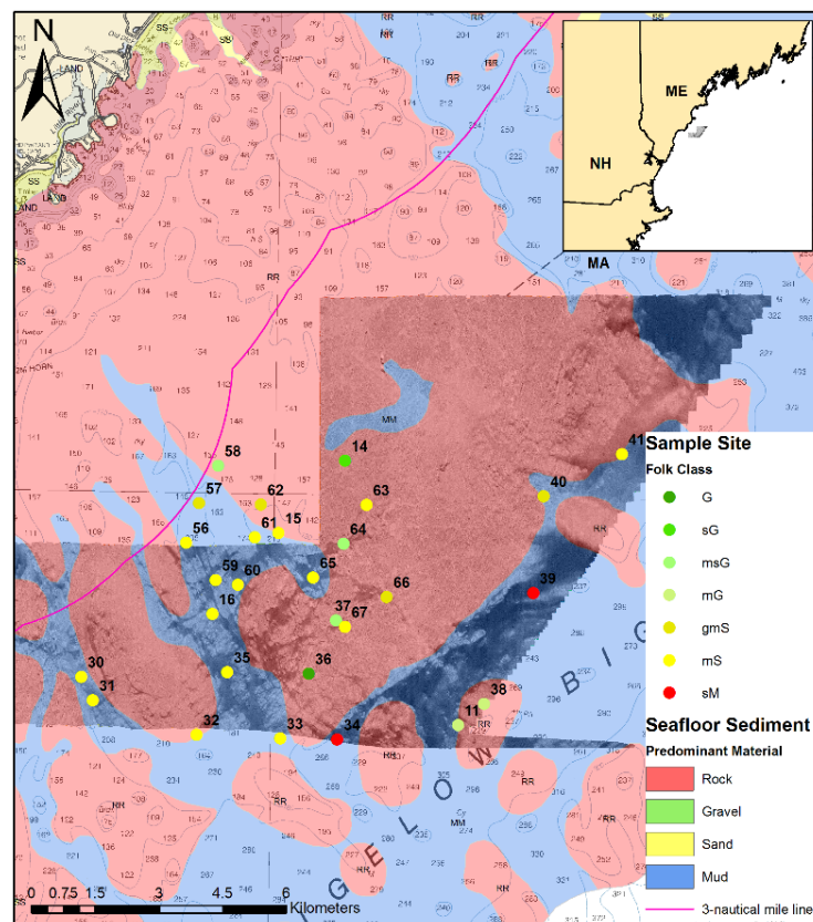
Figure 2. Generalized seafloor sediment map of the 2014 Kennebunk MCMC area showing interpreted extent of seafloor substrates (Barnhardt et al., 1998) and MCMC grab samples' Folk (1954) classification.
