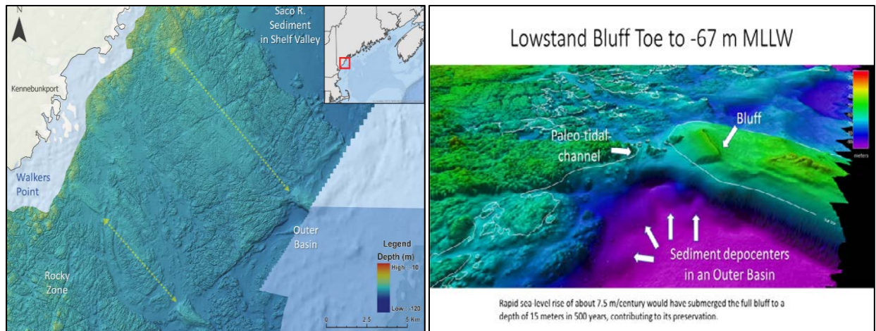
Figure 13. In the area of the MCMI's Kennebec MBES data collection, an esker truncated in a bluff with a base of slope from -60 to -67 m along a 220-m shoreline.
